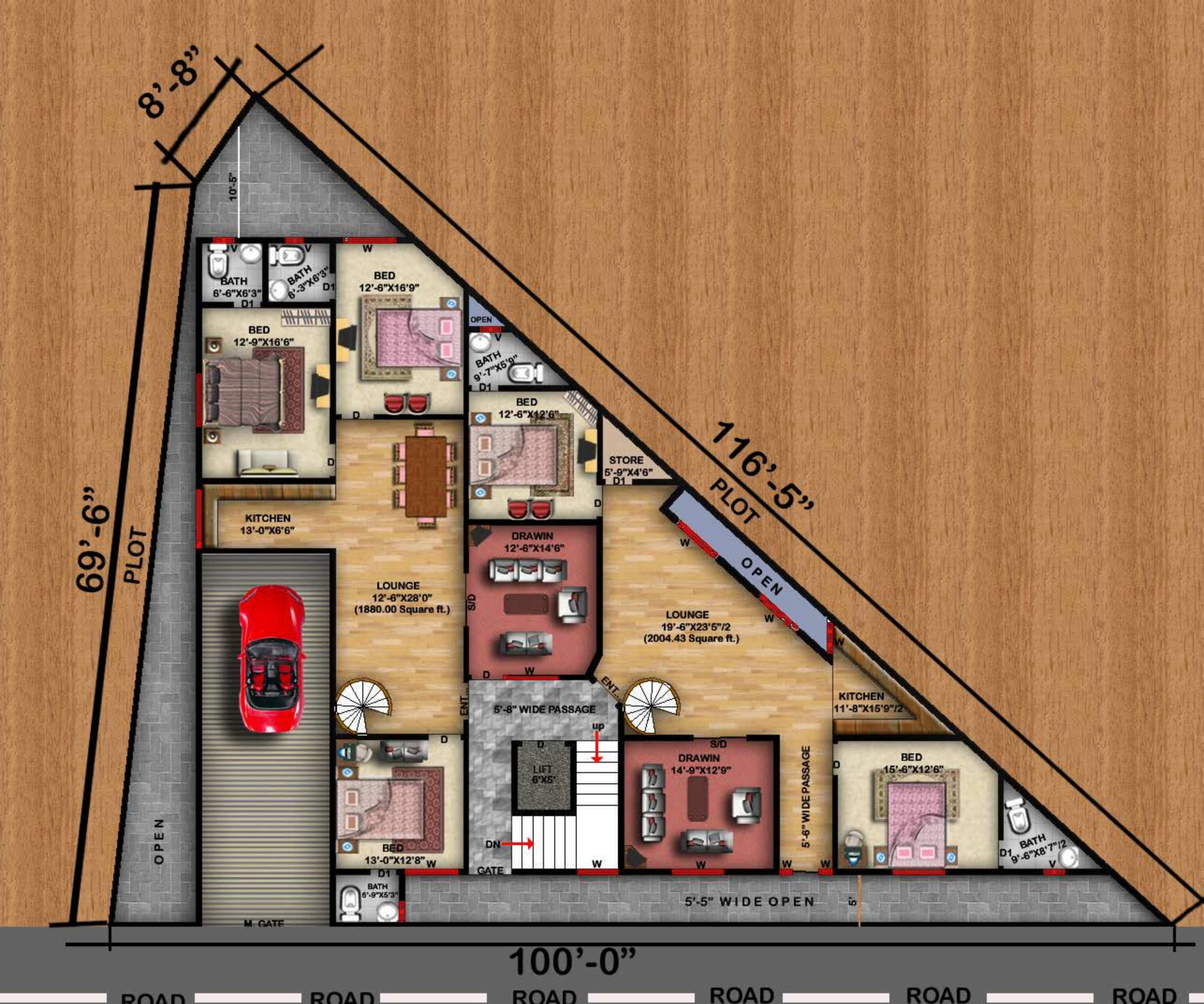
ROAD ROAD ROAD ROAD ROAD ROAD GROUND FLOOR PLAN
