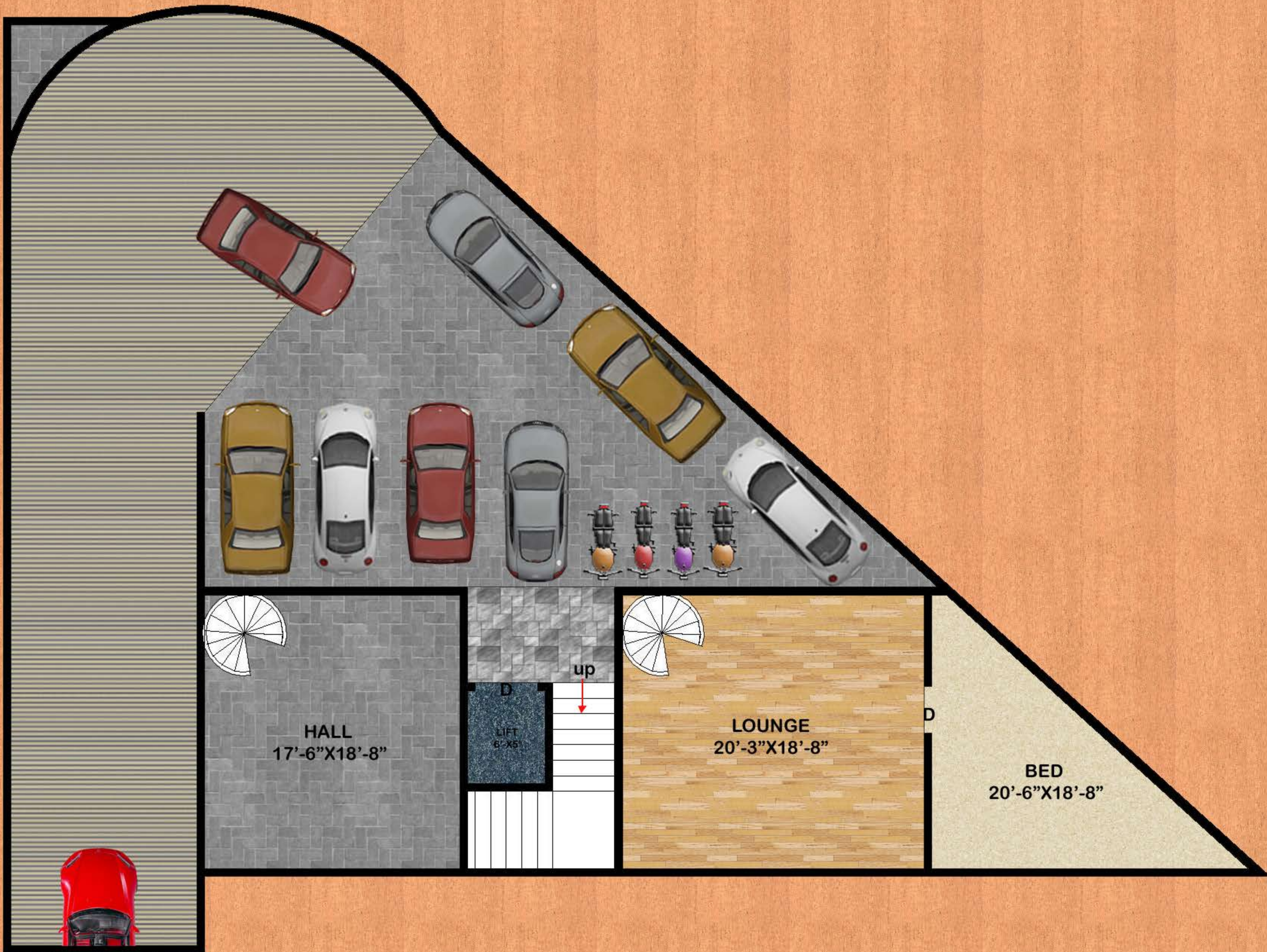
BASEMENT PLAN
